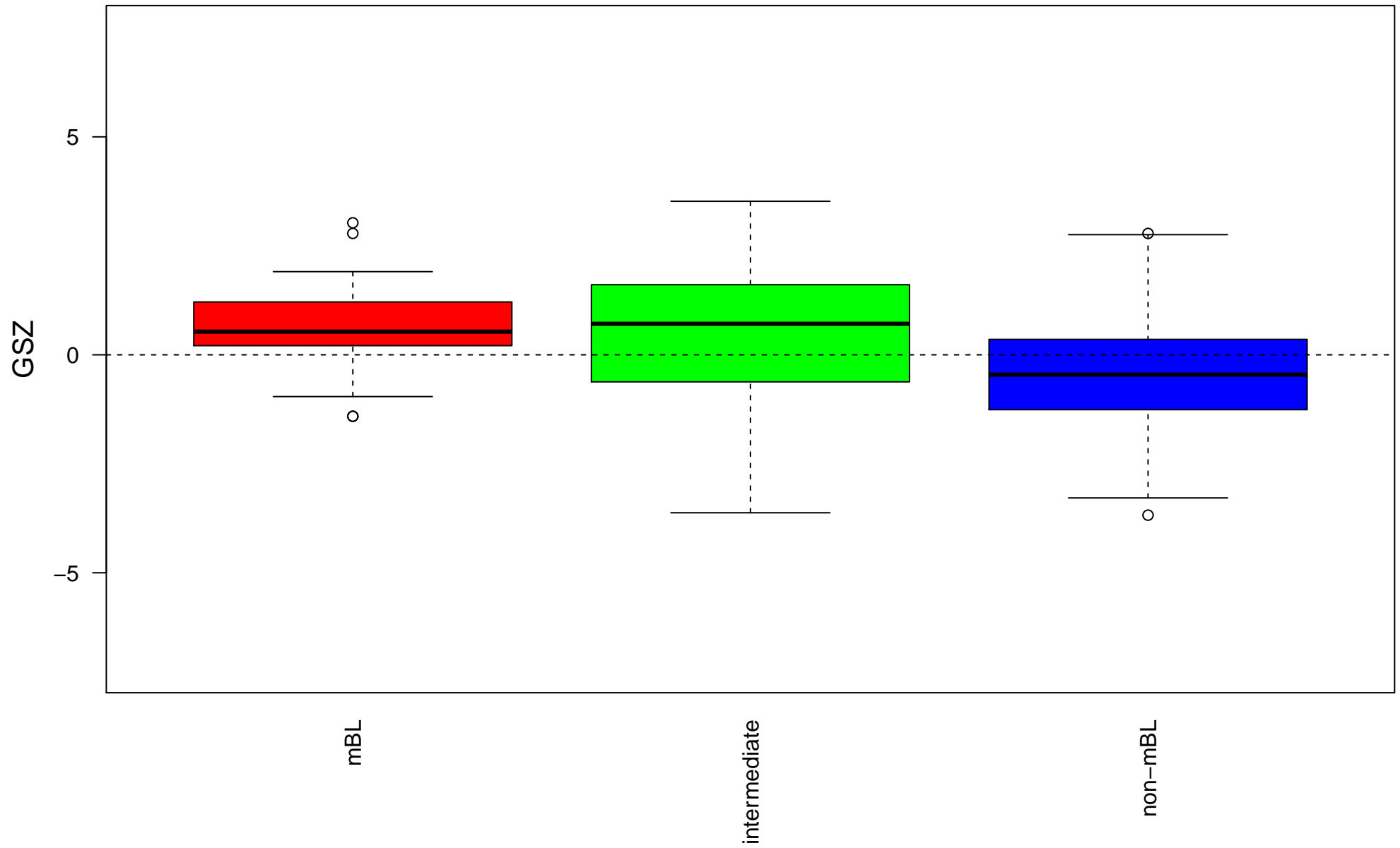
Pentrack_CRC_TCGA_corr_N_msi-h_DN
